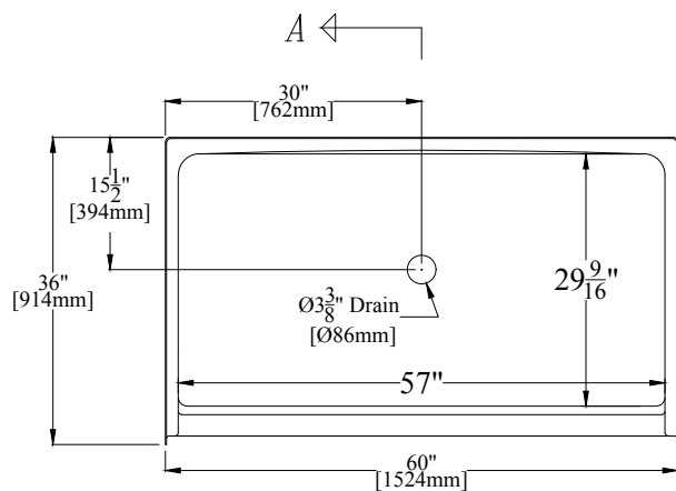
PLAN 60" [1524mm] Shower w/ 7" [178mm] Threshold
