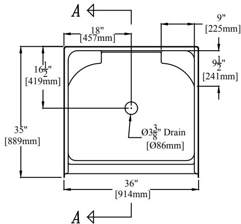
36" [914mm] Shower w/ 7" [178mm] Threshold & Molded Soap Ledges
